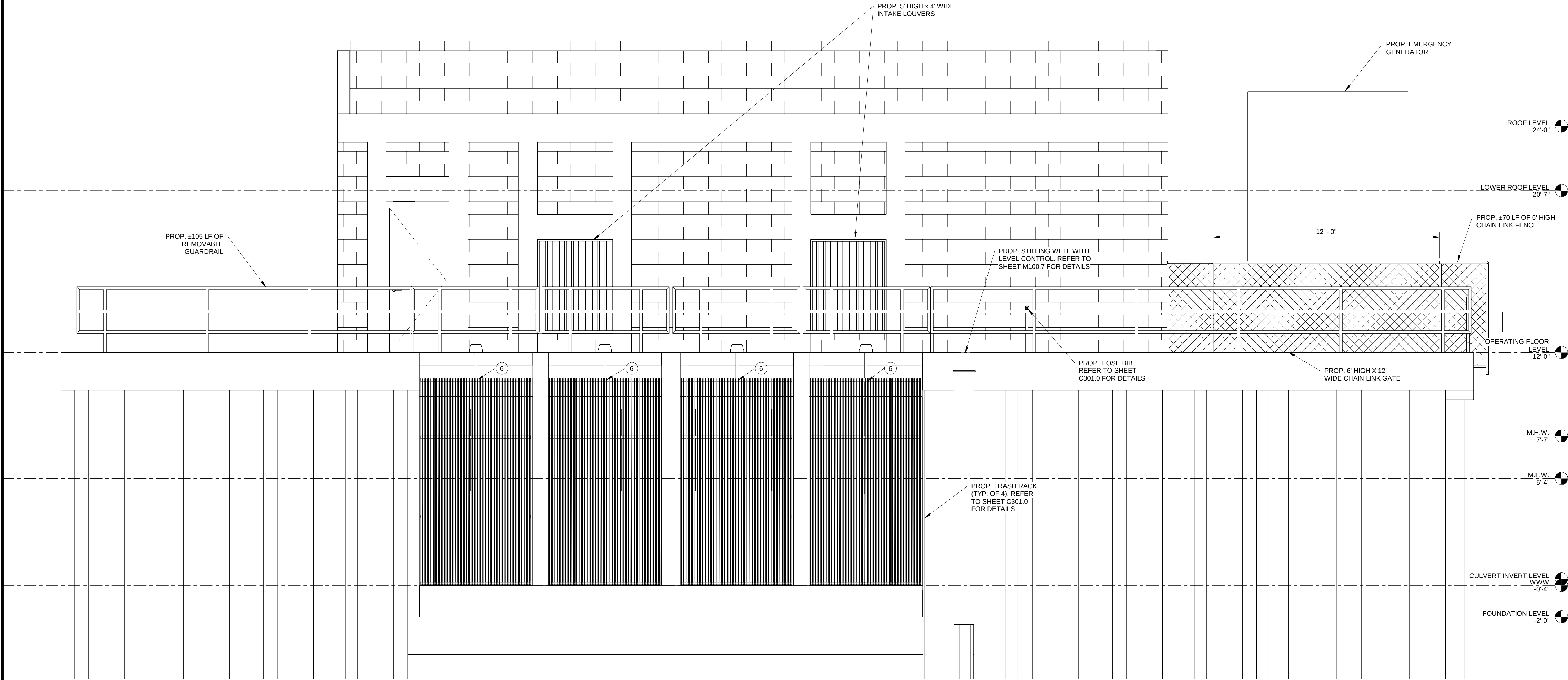
4 Section B-B 3/8" = 1'-0"
